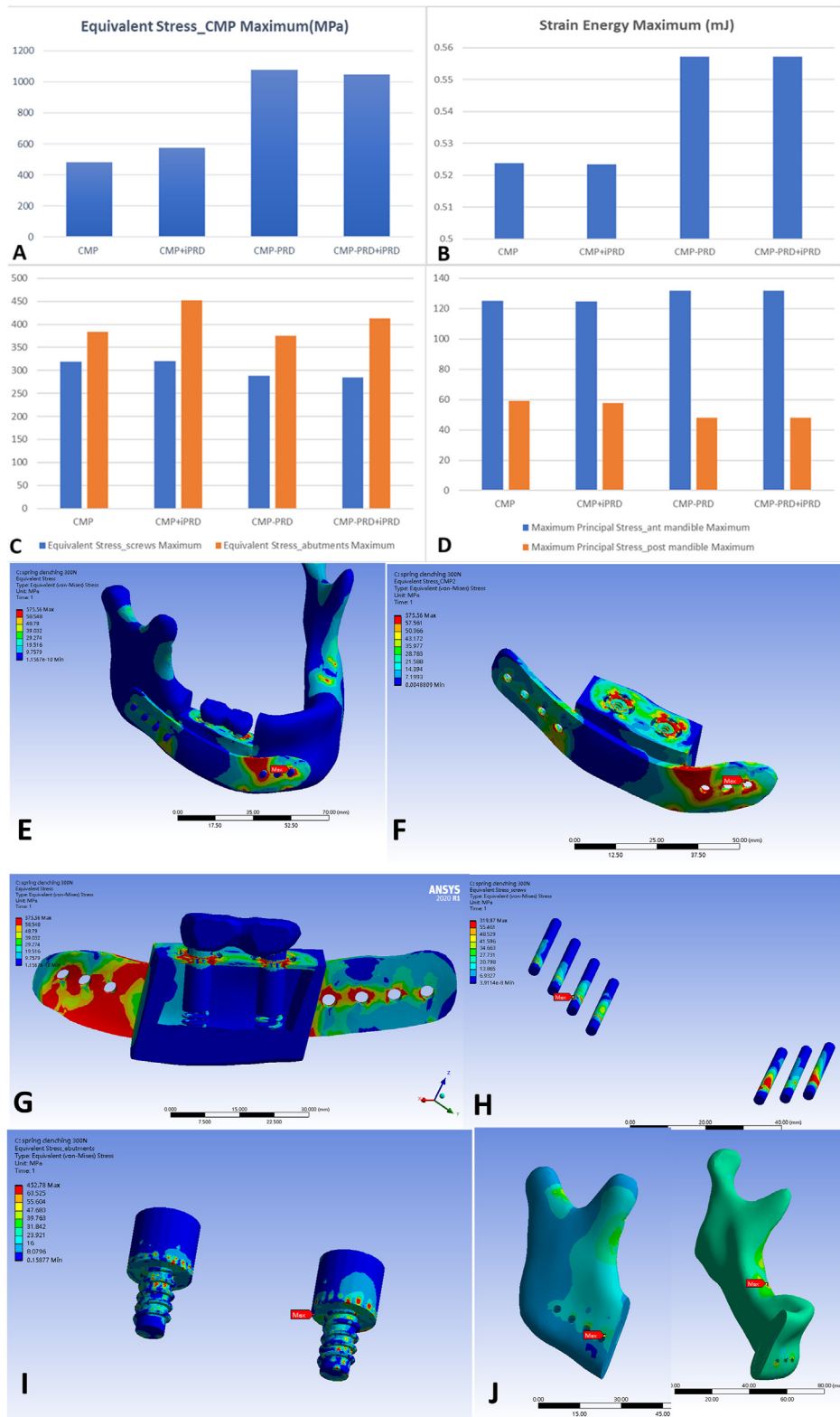
Figure 3 The maximum values of von Mises equivalent stress, strain energy, and von Mises equivalent principal stress in the 4 types of CMP. (A) Von Mises equivalent stress of the entire assembly. (B) Strain energy of the entire assembly. (C) Von Mises equivalent stress of retentive screws and abutments. (D) Von Mises principal stress of the anterior and posterior mandible. Von Mises equivalent stress of the entire assembly (E), CMP with iPRD (F), perspective view of CMP with iPRD (G), retentive screws (H), abutments (I), and anterior and posterior mandible (J). Abbreviations: CMP, customized mandible prostheses, PRD, pressure-reducing device, iPRD, implant pressure-reducing device.
