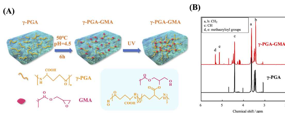
Figure 2 (A) Synthesis of \gamma -PGA hydrogel into \gamma -PGA-GMA, (B) NMR analysis for ^1\text{H} NMR spectrum of \gamma -PGA hydrogel with GMA.
