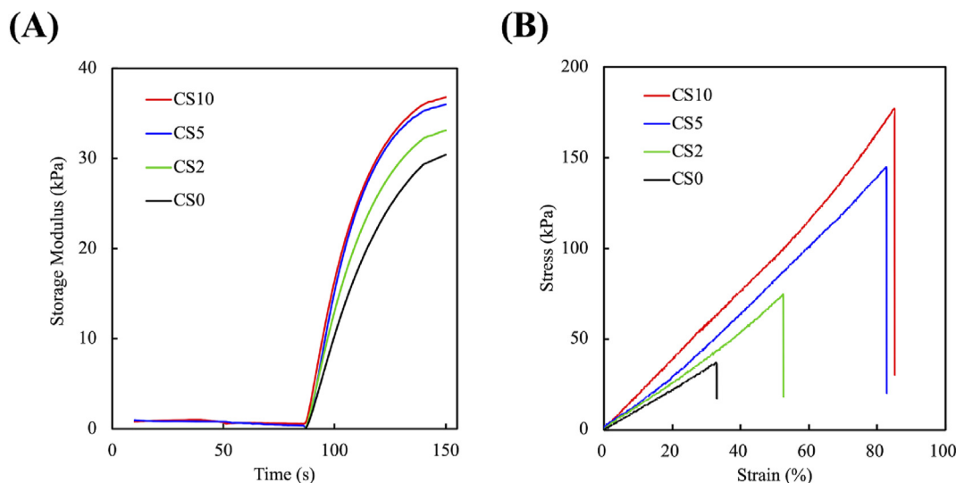
Figure 5 The evolution of (A) dynamic rheology properties and (B) stress-strain curve for CS0, CS2, CS5, and CS10 hydrogel. Data presented as mean \pm SEM, n = 6 for each group. (SEM, standard error of mean).
