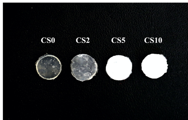
Figure 3 The morphology of \gamma -PGA-GMA/CS hydrogel with different calcium silicate (CS) concentrations. (CS0 = 0% CS; CS2 = 2% CS; CS5 = 5% CS; CS10 = 10% CS).
