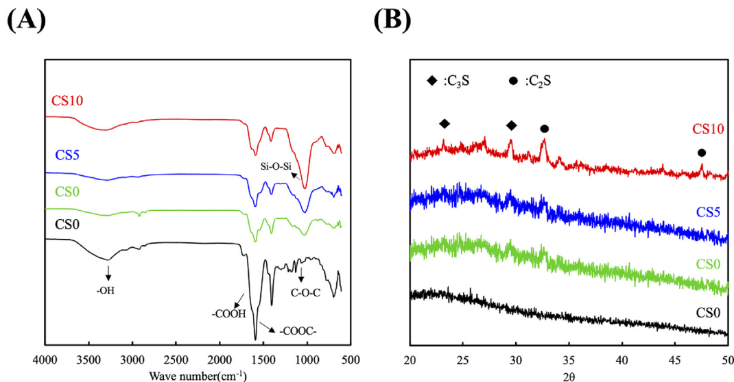
Figure 4 (A) The functional group of FTIR and (B) phase structure of XRD results for the different concentrations of calcium silicate (CS) contained \gamma -PGA-GMA hydrogel.
