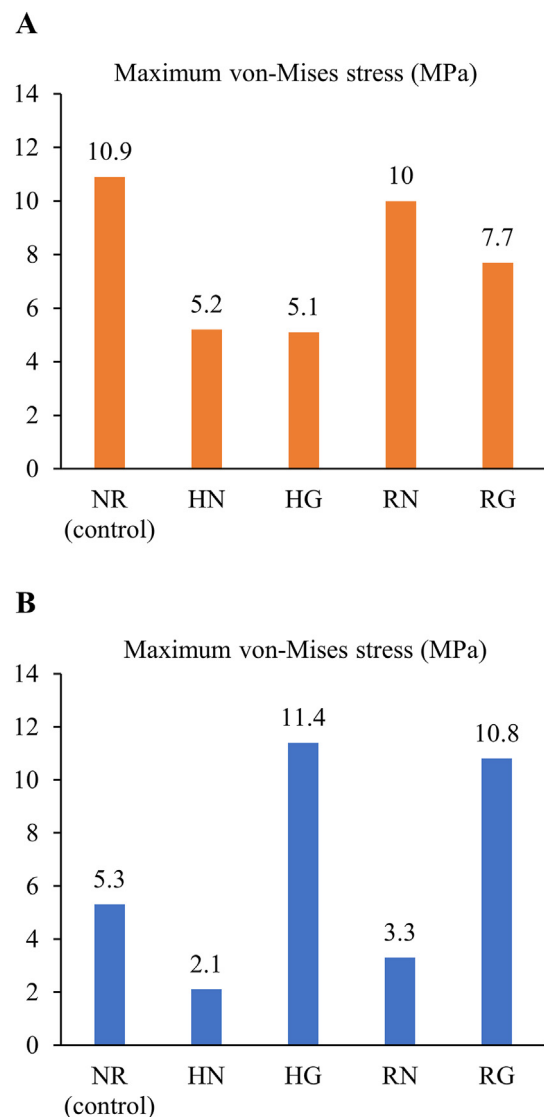
Figure 3 Maximum von-Mises stress values for each different model: (A) On the bone; (B) at the root apex.
