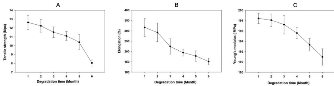
Fig. 2 The mechanical properties of a PCL (Polycaprolactone) scaffold with a 0 inner diameter of HTA (Half tubular array) follow hydrolytic degradation in phosphate buffered saline at 37 °C for 6 months. The mechanical properties were measured every month. The tensile strength steadily decreased from month 1 to month 4, and the value reduction was more evident and significant during months 5 and 6 (A). The maximum strain percentage decreased significantly during month 3, and the degradation rate decreased gradually up to 6 months (B). Young's modulus reduction with time dependence was observed without statistical significance (C). n = 6-8 , *P < 0.05 .
