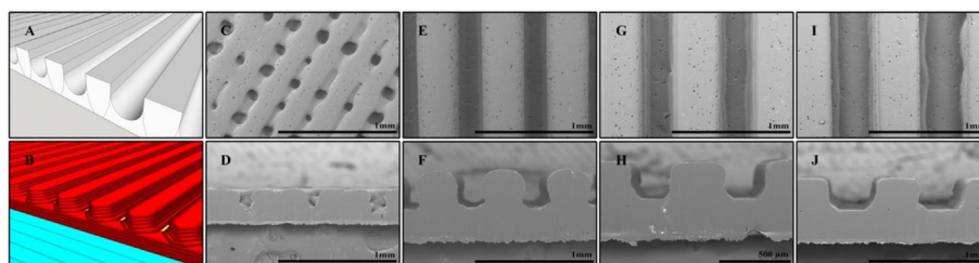
Fig. 1 3D design of PCL scaffold with a 200- \mu\text{m} inner diameter of HTA (A). 3D-slicing of PCL scaffold (B). Top view of 3D-printed PCL scaffold with 0, 200, 300, and 400 \mu\text{m} inner diameters of HTA (C.E.G.I). Cross-section of 3D-printed PCL scaffold with 0, 200, 300, and 400 \mu\text{m} inner diameter of HTA (D.F.H.J). PCL: Polycaprolactone; HTA: Half tubular array.
