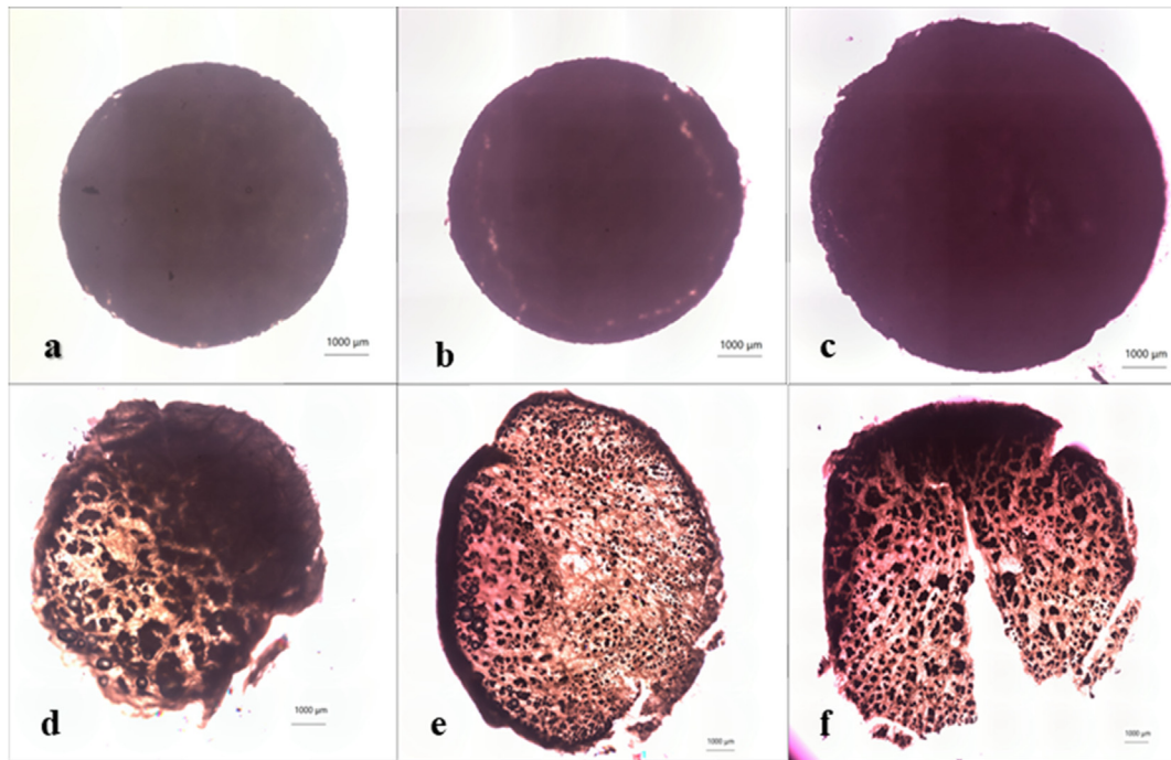
Figure 1 Solubility of fish gelatin-/porcine gelatin-derived 2:2 G-HAp membranes. a-c: fish gelatin-derived G-HAp membranes in culture medium at 24 h (a), 3 days (b), and 5 days (c). d-f: porcine gelatin-derived G-HAp membranes in culture medium at 24 h (d), 3 days (e), and 5 days (f).
