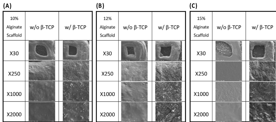
Figure 3 SEM images of 3D-printed scaffolds at different alginate concentrations: (A) 10, (B) 12, (C) 15 wt%, alginate, and alginate/β-TCP particles. Images are presented at four different magnifications (X30, X250, X1000, X2000) to highlight structural details. SEM: Scanning Electron Microscope; β-TCP: β-tricalcium phosphate.
