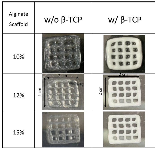
Figure 2 Macroscopic images of 3D-printed at different alginate concentrations, alginate alone or alginate/β-TCP (dimensions: 2 cm*2 cm). Images depict the geometry immediately after printing and after undergoing a 10-min cross-linking process in a CaCl 2 bath. β-TCP: β-tricalcium phosphate.
