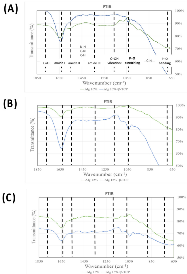
Figure 4 FTIR: Fourier-transform infrared spectroscopy spectra of the bioprinting scaffold and its individual components. (A) Alg 10 % and Alg 10 %+ \beta -TCP (B) Alg 12 % and Alg 12 %+ \beta -TCP (C) Alg 15 % and Alg 15 %+ \beta -TCP. FTIR: Fourier-Transform Infrared Spectroscopy.
