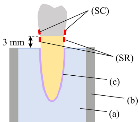
Figure 3 Schematic representation of the embedded experimental specimens. (a) Acrylic resin, (b) Aluminum ring, (c) Vinyl polysiloxane impression material, (SC) Strain gauge attached to crown, and (SR) Strain gauge attached to root.
