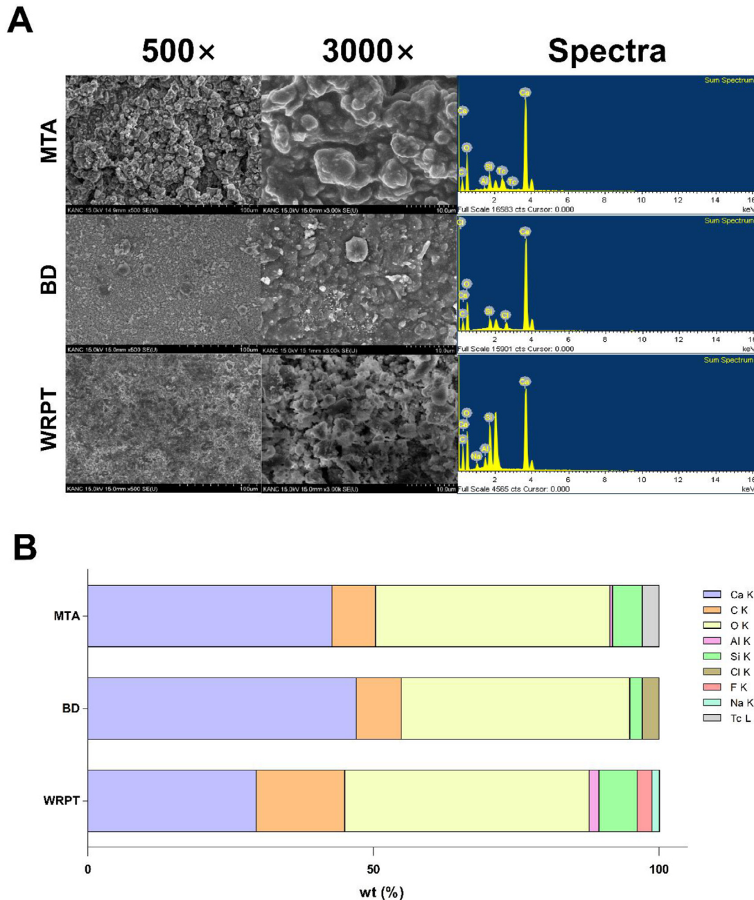
Figure 2 Scanning electron microscopy/energy-dispersive spectroscopy (SEM-EDS) mapping. (A) Representative SEM images with 500 × and 3000 × magnifications and the corresponded EDS spectra. (B) The weight volume (%) of the components. Note that the calcium volume was the highest in BD, followed by MTA and WRPT. MTA, mineral trioxide aggregate; BD, Biodentine; WRPT, Well-Root PT.
