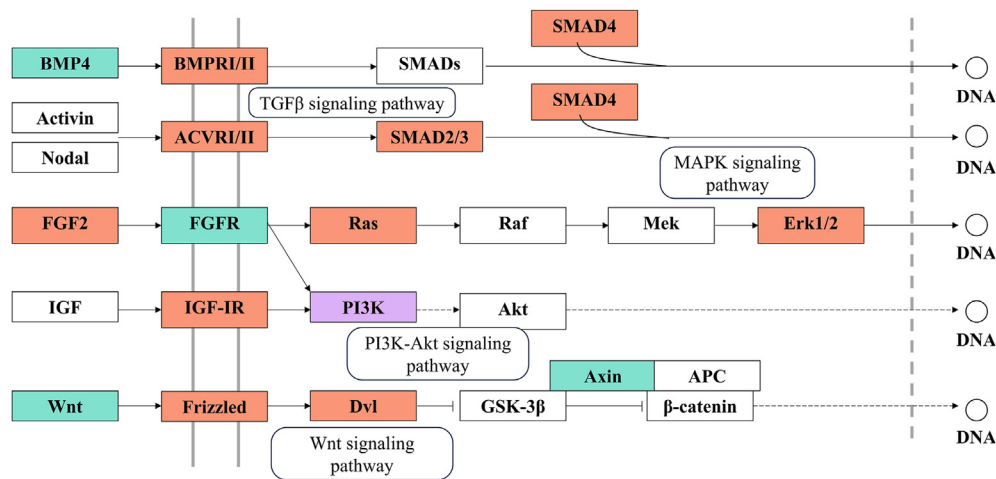
Figure 3 A section of “Signalling pathways regulating pluripotency of stem cells” as represented by KEGG. As it can be observed, this pathway is interconnected with “Wnt” and “TGFβ signaling” pathways, known to be related to odontogenesis. In light blue are reported tooth anomalies-associated genes, in orange miRNA’s target genes and in purple the genes belonging to both sets of genes.
