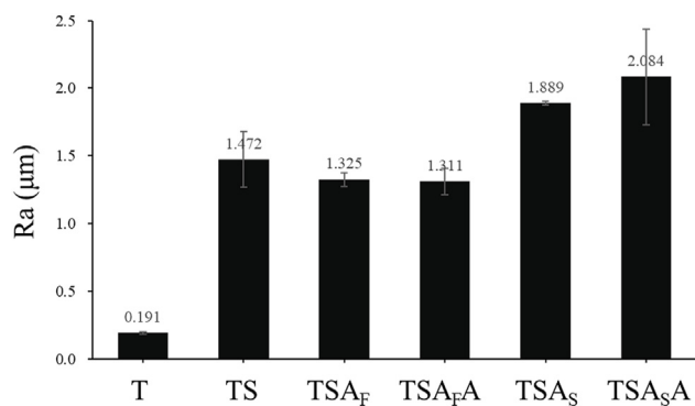
Figure 2 Surface roughness of all samples as indicated by \alpha -step. T: grade 4 Ti; TS: T discs underwent sandblasting; TSA F : the TS disks were etched in an acid bath of HNO 3 /HF; TSA 5 : the TS disks were etched in an acid bath of HCl/H 2 SO 4 ; TSA, TSA FA and TSA 5A : the TS, TSA F , and TSA 5 samples were soaked in NaOH.
