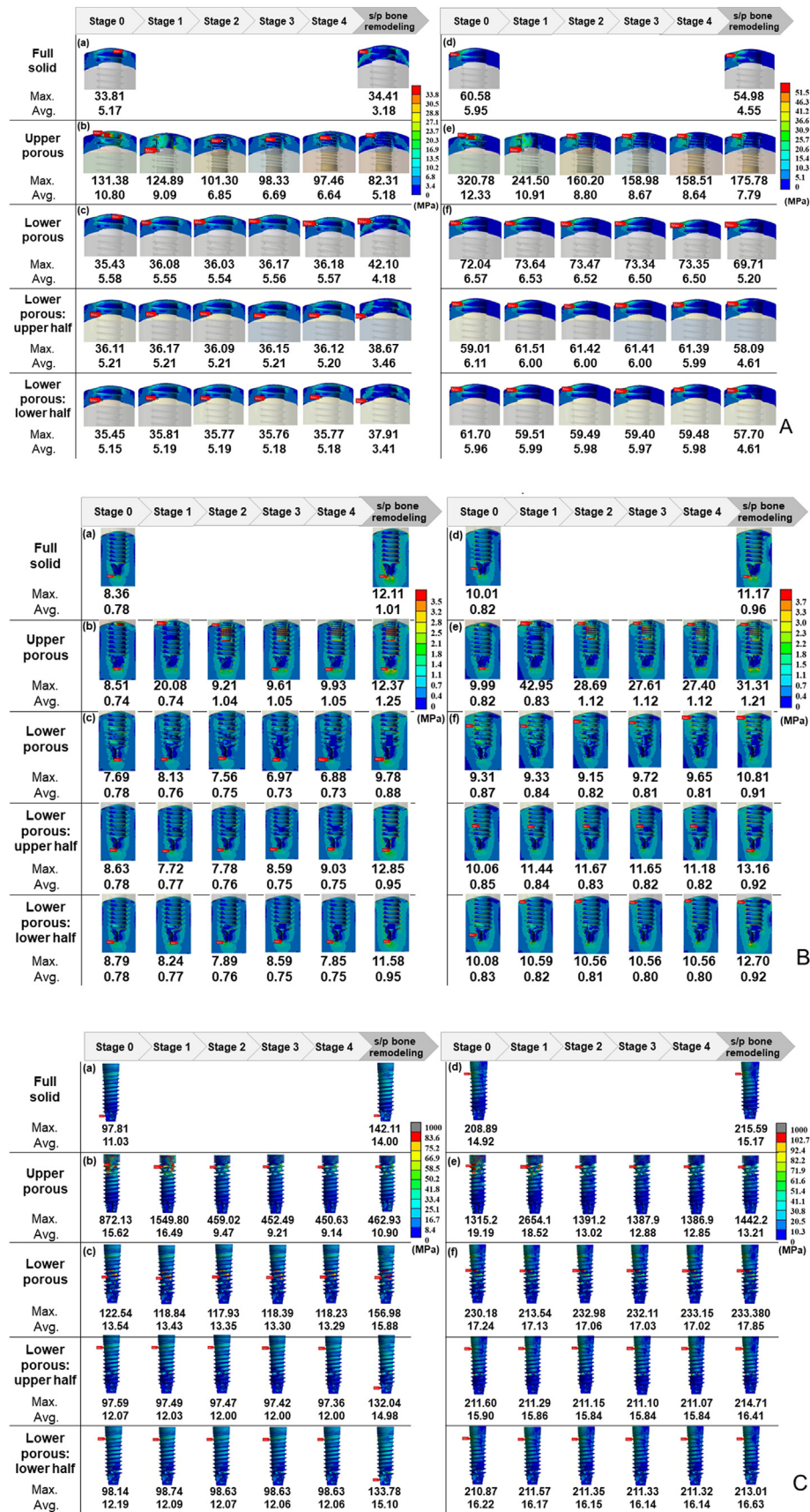
Figure 3 Maximum and average stress distribution in cortical bone (A), cancellous bone (B) and implant body (C). A: Maximum and average stress distribution in cortical bone, encompassing Stages 0–4 and post-surgery (s/p) bone remodeling.
